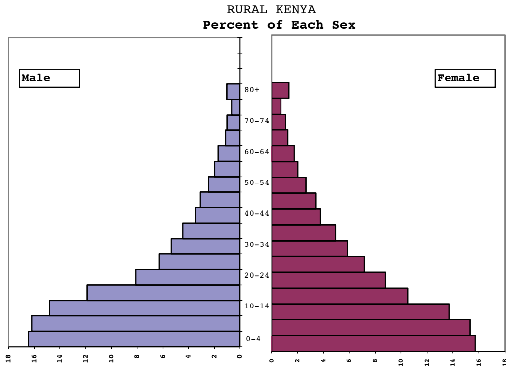
Figure 3: Population Pyramid, Rural Kenya 2009
