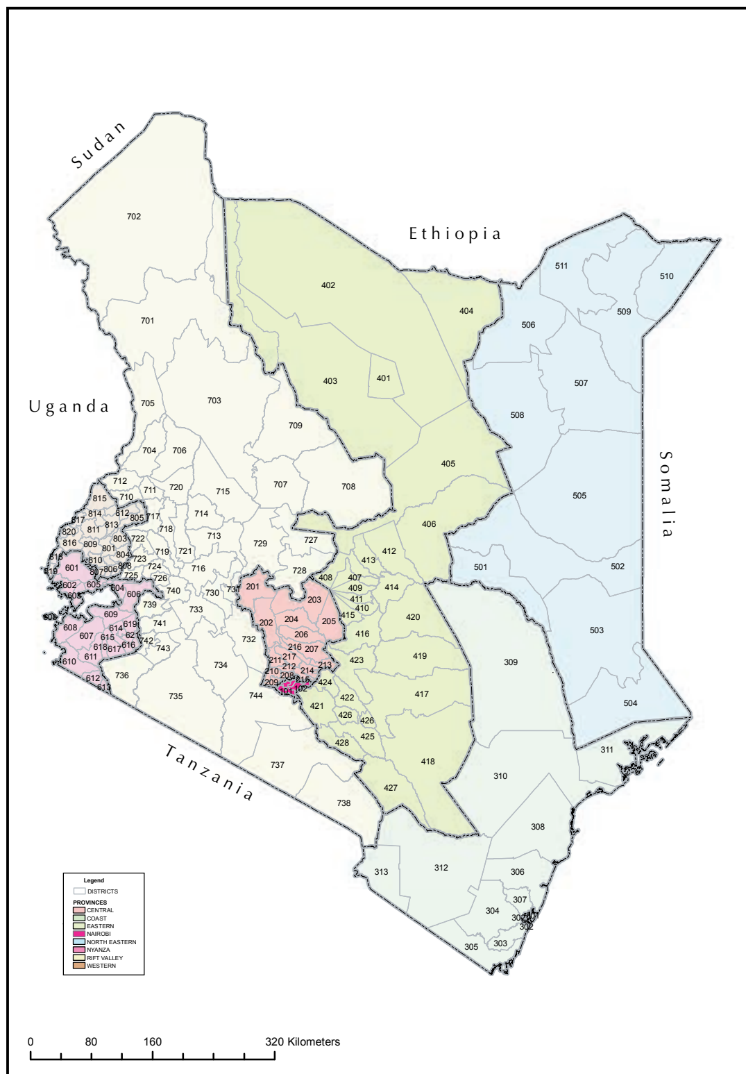
Figure 1: Kenya Administrative Units (December 2008)
