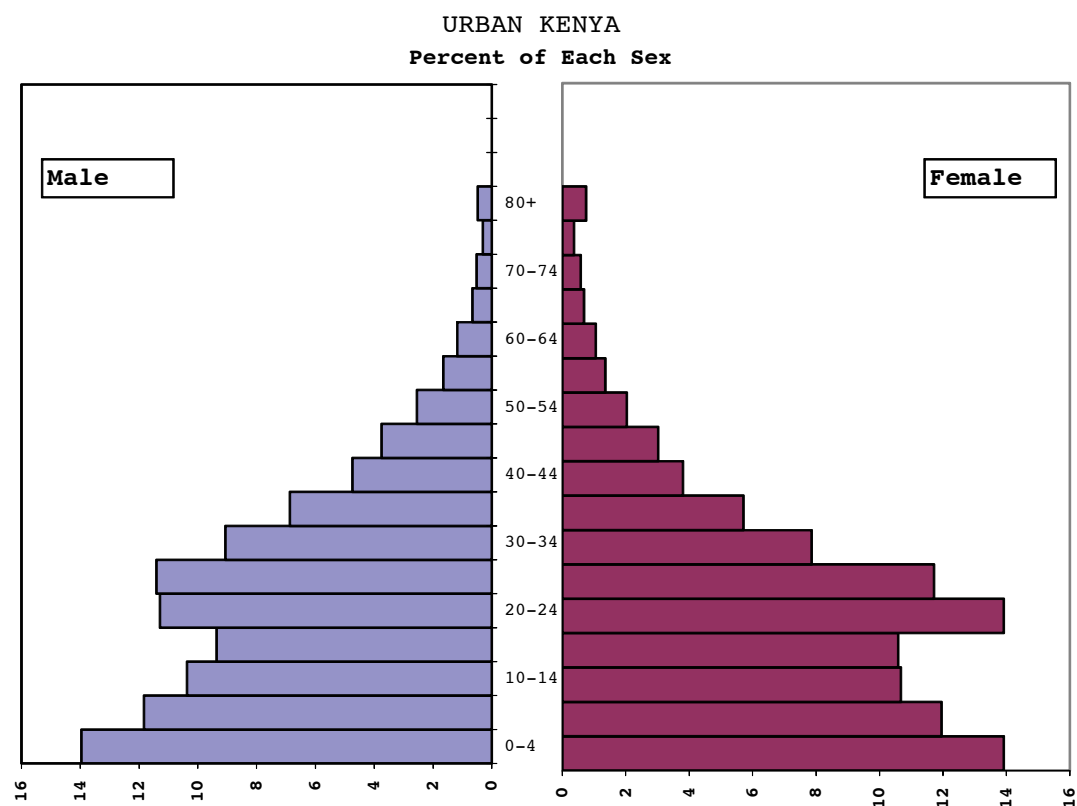
Figure 4: Population Pyramid, Urban Kenya 2009
